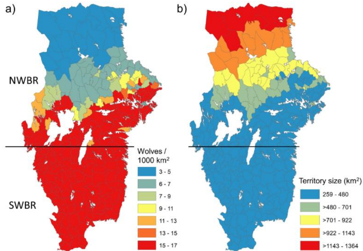
Figure 3. Predictions on wolf numbers and territory sizes obtained in the Swedish wolf breeding range (WBR), divided as north (NWBR) and south (SWBR). (a) Estimated number of wolves per 1000 km 2 obtained from the number of wolf territories that the abundance of deer prey (roe deer, red deer, fallow deer) can sustain per municipality and considering that a wolf territory contains on average 4.26 wolves in Scandinavia [63]. (b) Estimated wolf territory size (km 2 ) per municipality as a function of deer density and latitude as modelled in Mattisson et al. [63].
